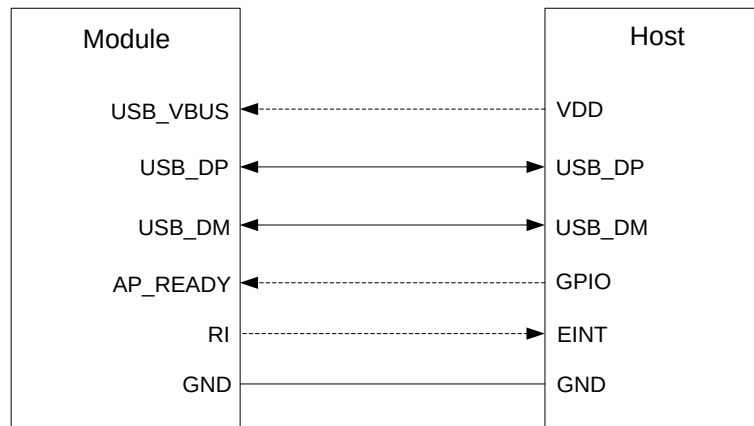
Figure 4: Connection Diagram Based on USB Suspend/Resume and RI Pin
