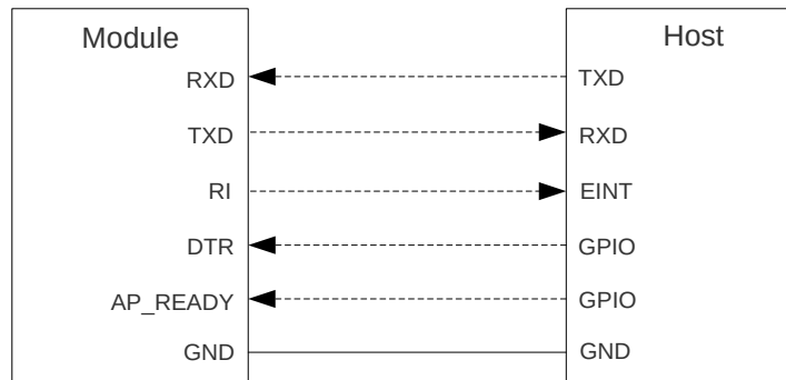
Figure 1: Connection Diagram Based on UART
