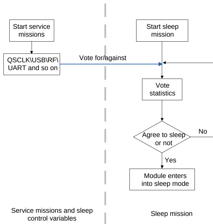
Figure 5: Sleep Process
