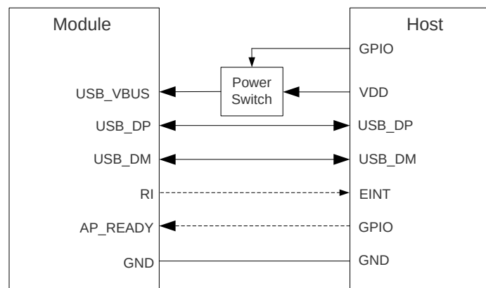
Figure 3: Connection Diagram Based on USB Disconnection
