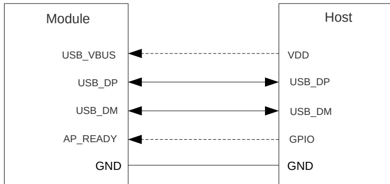
Figure 2: Connection Diagram Based on USB Remote Wakeup
